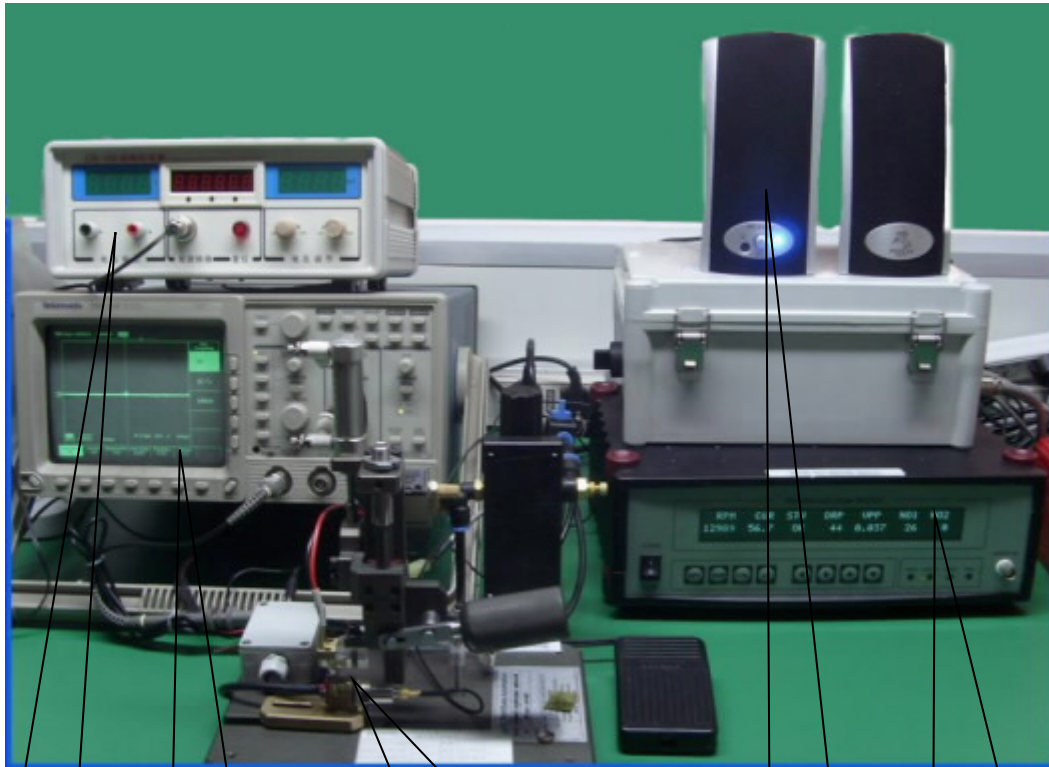
启动测试仪 Start-Work Test Meter
