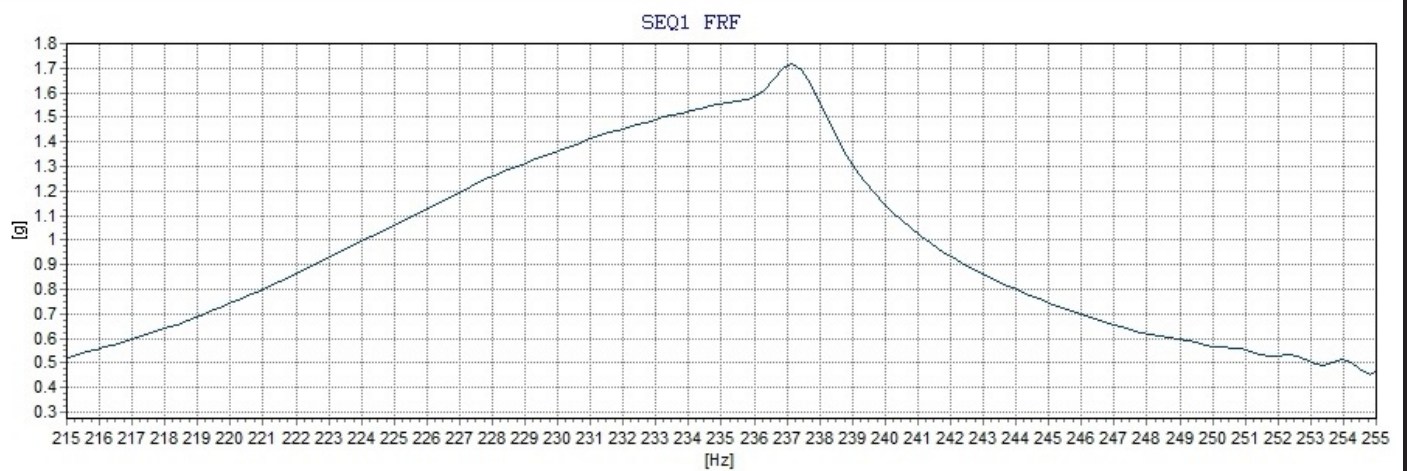
Frequency VS. Acceleration Characteristics
